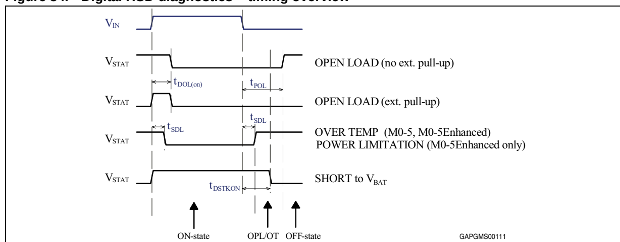
Figure 34. Digital HSD diagnostics – timing overview
