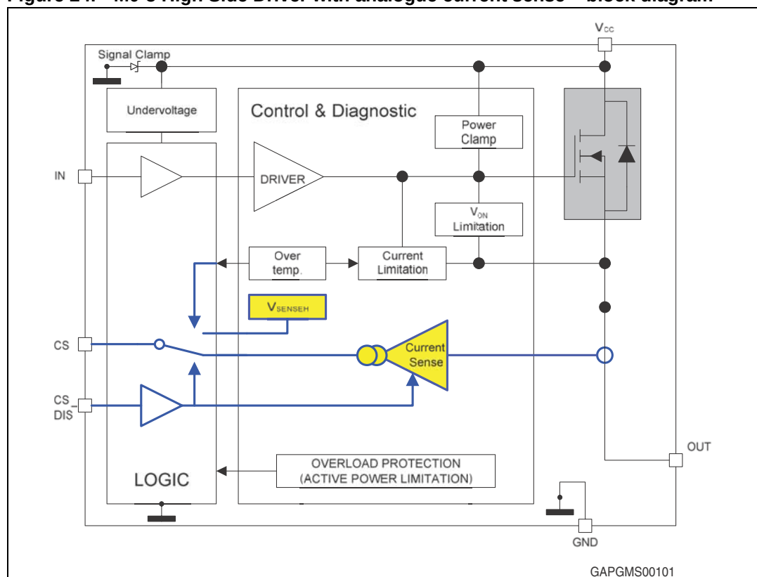
Figure 24. M0-5 High Side Drive with analogue current sense – block diagram
