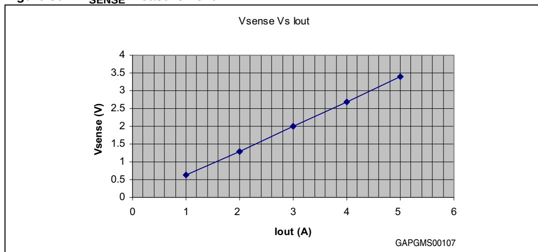
Figure 30. V_{SENSE} measurement
