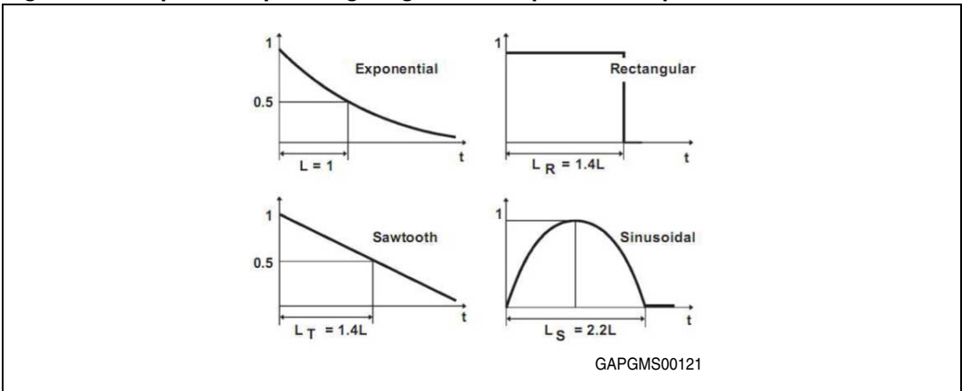
Figure 45. Equivalent pulses giving the same power dissipation
