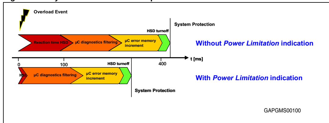
Figure 23. System reaction time comparison
