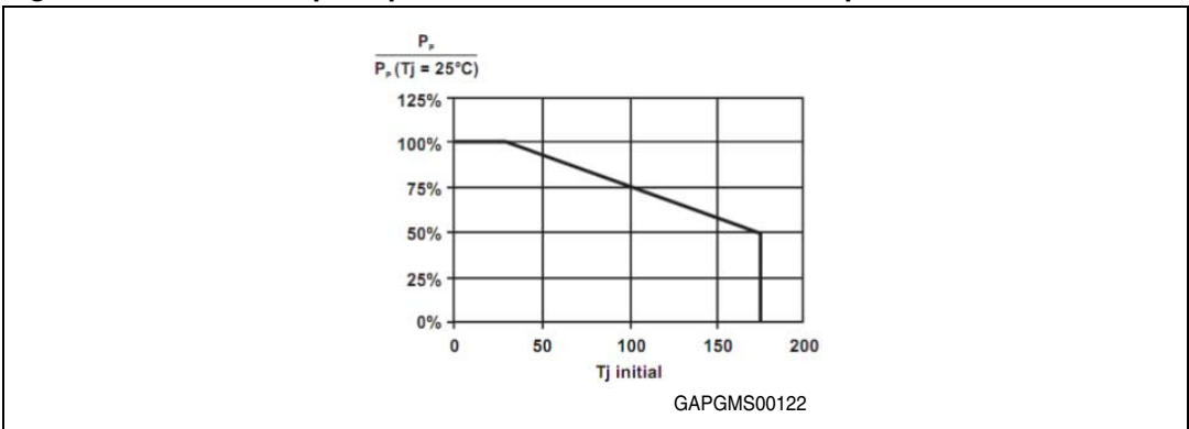
Figure 46. Maximum peak power as a function of initial temperature of the transil
