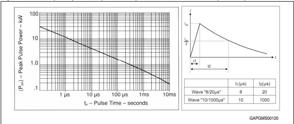
Figure 44. Peak pulse power vs pulse time (for transil 600 W@10/1000 \mu s series)
